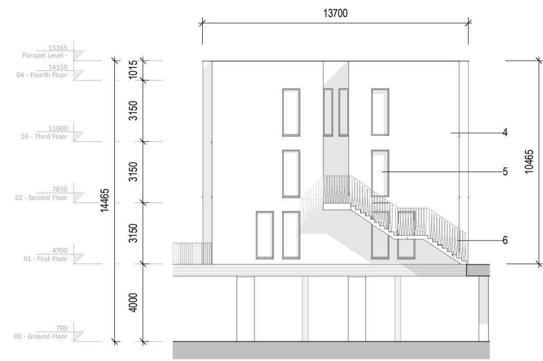
2 A2_Duplex North-East Elevation 1:200
