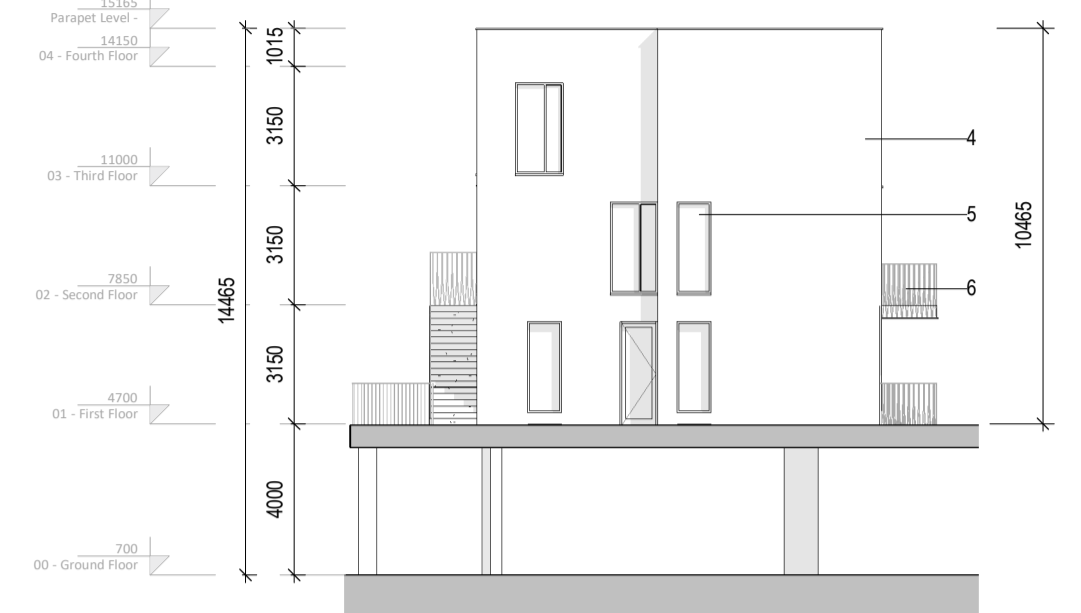
4 A2_Duplex North-West Elevation 1:200
