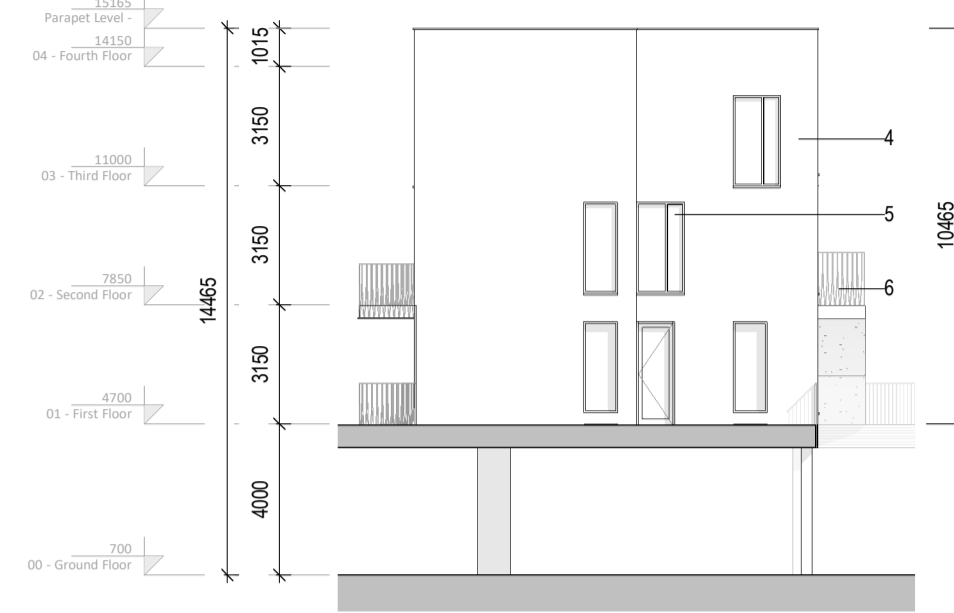
3 A2_Duplex East-South Elevation 1:200
